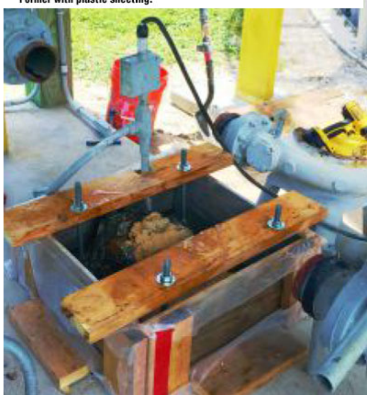
Bolt placement guides.
